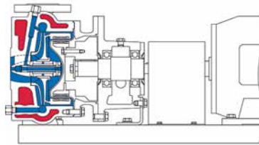
Frame-mounted MKP with heating with baseplate -100°C to +250°C
