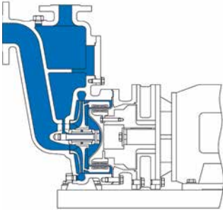
Close-coupled MKP-S with baseplate -100°C to +250°C
