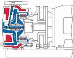
Close-coupled MKP with heating with baseplate -100°C to +250°C
