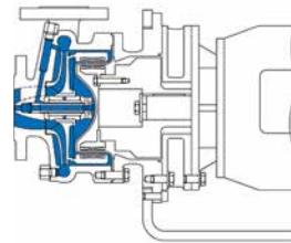
Close-coupled MKP with bracket -100°C to +250°C
