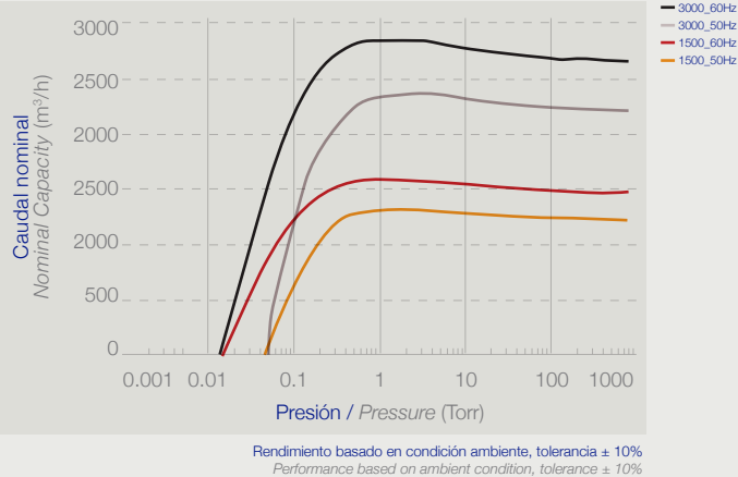
Curvas de caudal / Flow curves RVS-1500/3000
