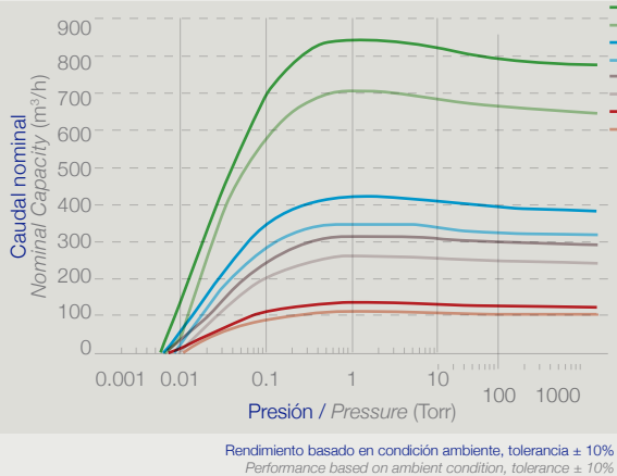
Curvas de caudal / Flow curves RVS-150/300/400/800
